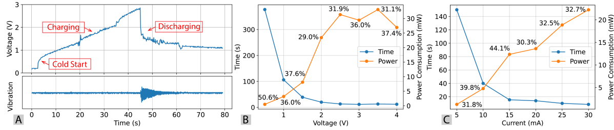
Fig. 10. System validation results. (A) top shows an example capacitor charging curve with 3V, 10mA input, while bottom shows the corresponding vibration magnitude measured by the vibration sensor. The right two plots show the charging duration, power consumption, and power efficiency with different input voltages (B) and currents (C). The % number next to each data point of the orange curve is the energy conversion efficiency at the corresponding condition.
