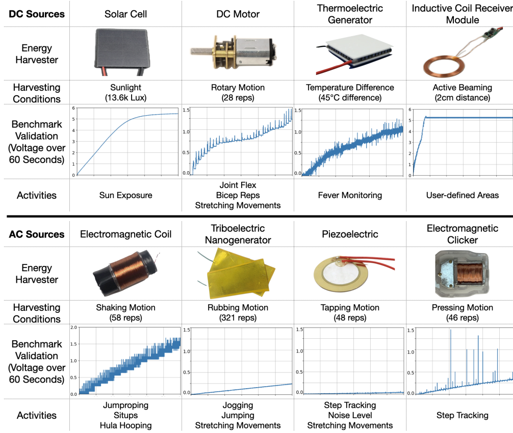
Fig. 9. Two tables detailing the energy harvesting inputs we tested; top table is DC sources and bottom table is AC sources. Harvesting Conditions are the evaluation conditions that correspond to the charge over time data in the Benchmark Validation row. To acquire this data, we connected the rectified harvesters to a 0.047F supercapacitor. We attached these harvesters to optimal locations on a user and repeated the associated activity, recording the number of repetitions while monitoring the capacitor's voltage over time. This allows us to visualize the distinct charging characteristics of different energy sources to inform our application design, and to evaluate the feasibility of these energy harvesters for Hapt-Aids.
