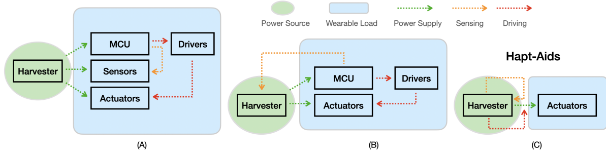
Fig. 5. Design options for self-powered activity monitoring device with haptic actuation. (A) Systems with energy harvesters, an MCU, and peripheral devices including sensors, drivers, and haptic actuators. (B) Systems with energy harvesters, an MCU that samples energy patterns for sensing (no peripheral sensors), drivers, and haptic actuators. (C) Our system (Hapt-Aids) utilizes analog components so that it has no peripheral sensors, drivers, or MCUs, only energy harvesters and actuators.
