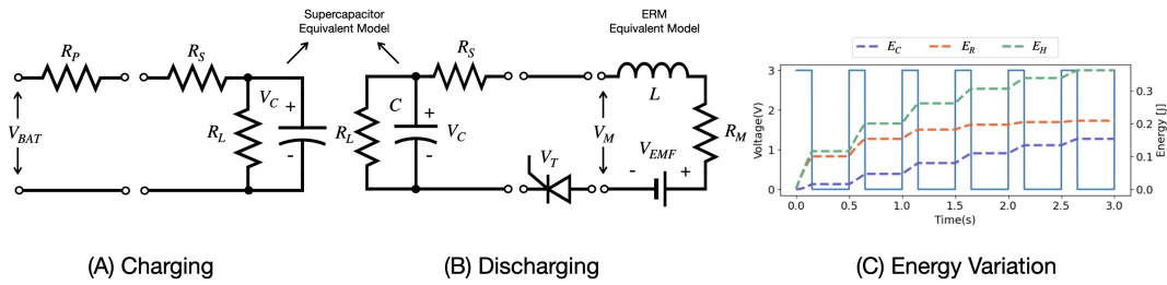
Fig. 6. Equivalent models of (A) charging and (B) discharging. R_p is resistance of the potentiometer. R_s and R_L are the equivalent series resistance and leakage resistance of the supercapacitor. The SCR triggers the discharging process at voltage V_T . R_M , L , and V_{EMF} are the resistance, inductance, and back EMF of the motor, respectively. The plot on the right (C) shows how the energy charged to the supercapacitor E_C increases approximately linearly with the number of input pulses.
