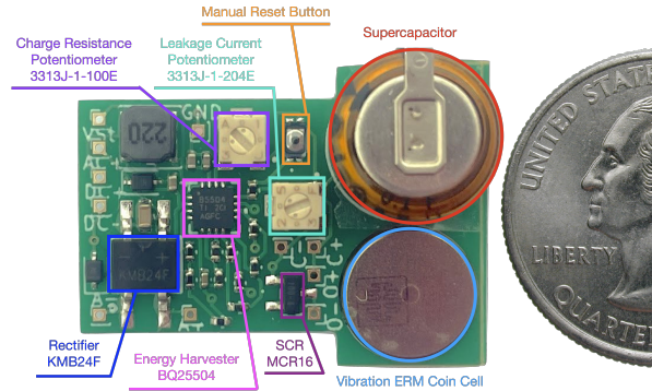
Fig. 8. Detailed shot of our custom PCB; we include a quarter for size comparison.
