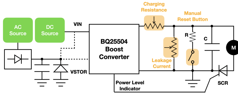
Fig. 7. A high-level overview of our entire system. For detailed implementation, see Figure 8.
